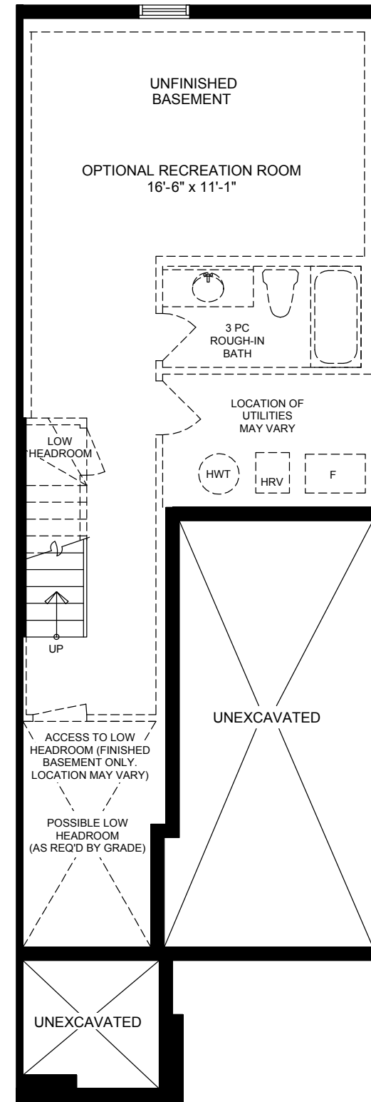
Basement Plan Elevation A & B
