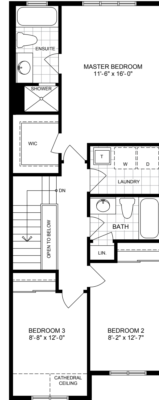
Second Floor Plan Elevation A
