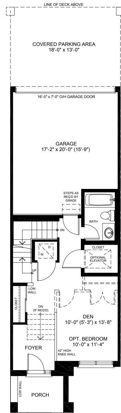
Ground Floor Plan Elevation A
