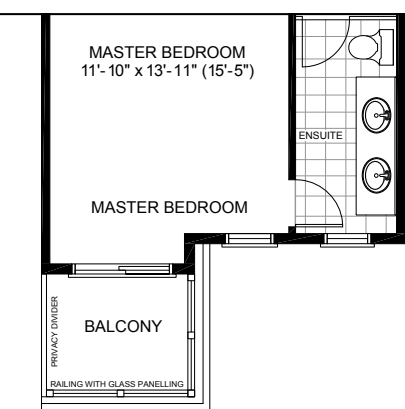
Partial Upper Level Floor Plan Elevation B
