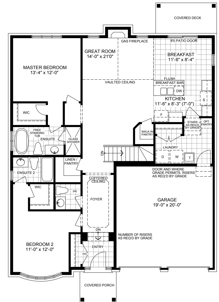
Optional Ground Floor Plan Elevation A
