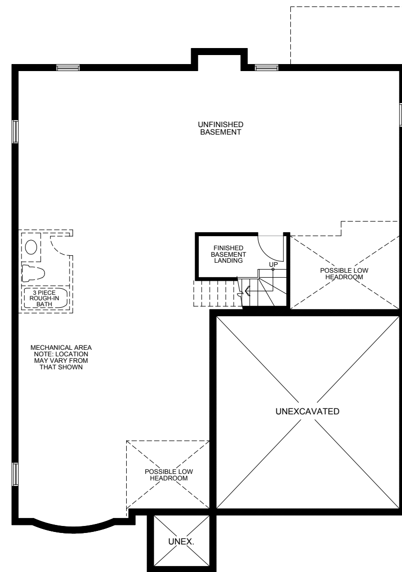
Basement Plan Elevation A
