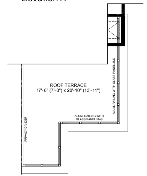
Roof Terrace Plan Elevation A
