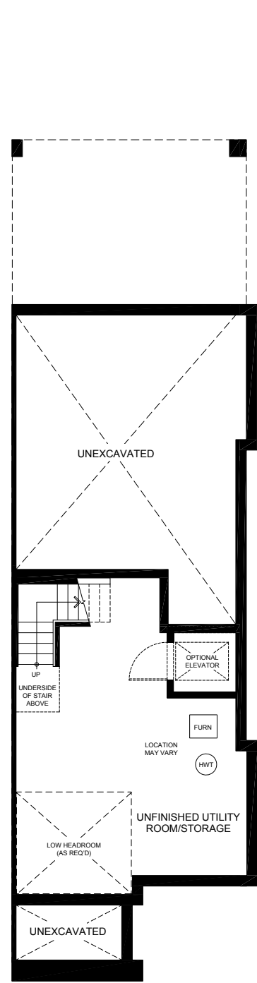
Basement Plan Elevation A & B
