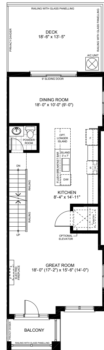
Main Floor Plan Elevation A
