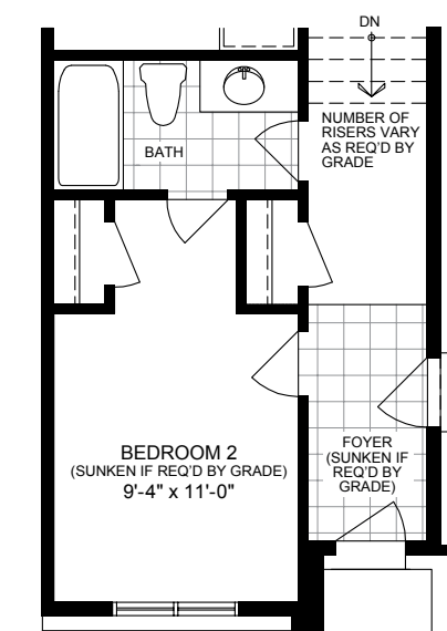
Partial Ground Floor Plan with optional shared bathroom
