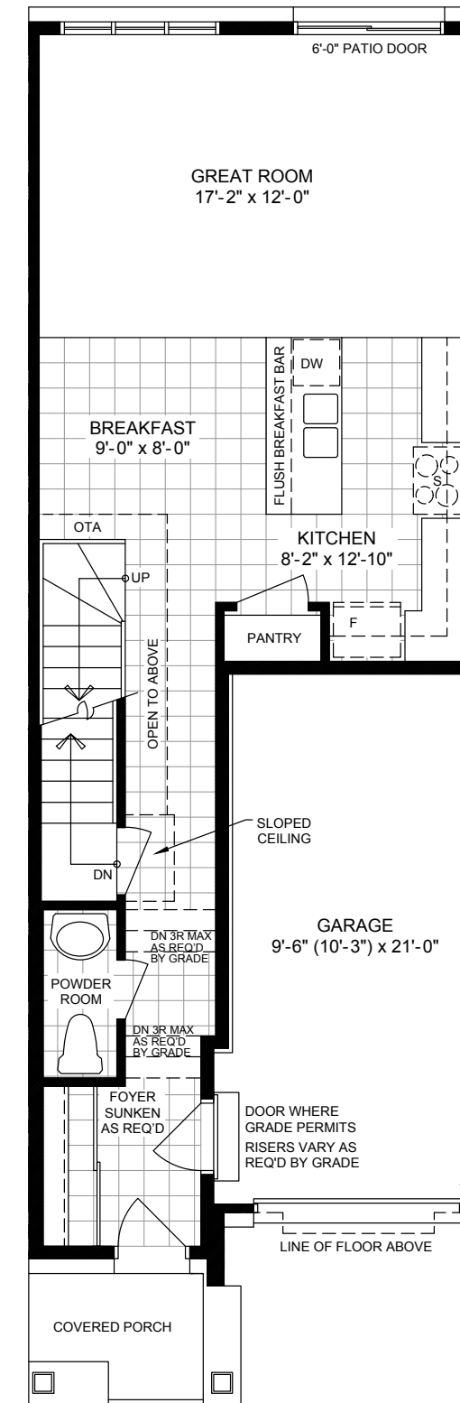
Ground Floor Plan Elevation A & B
