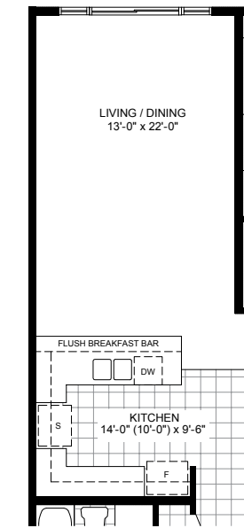
Partial Ground Floor Plan with Optional Kitchen Layout with Optional Powder Room at Landing
