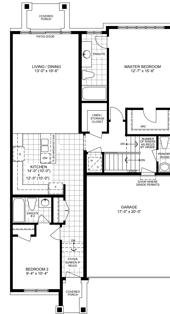
Ground Floor Plan with Optional Powder Room at Landing
