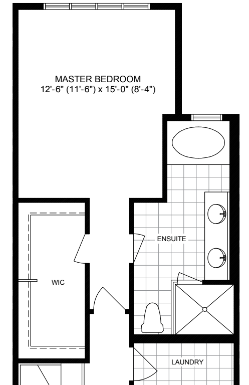
Partial Optional 3 Bedroom Second Floor Plan with Enlarged Master Ensuite Elevation A & B
