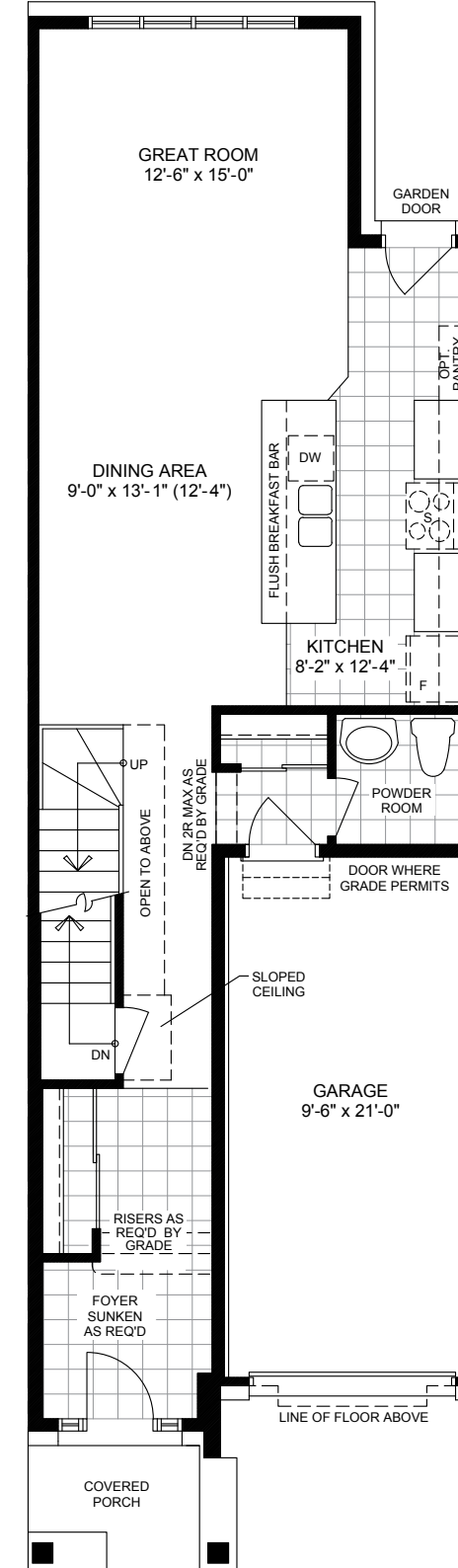
Ground Floor Plan Elevation A & B
