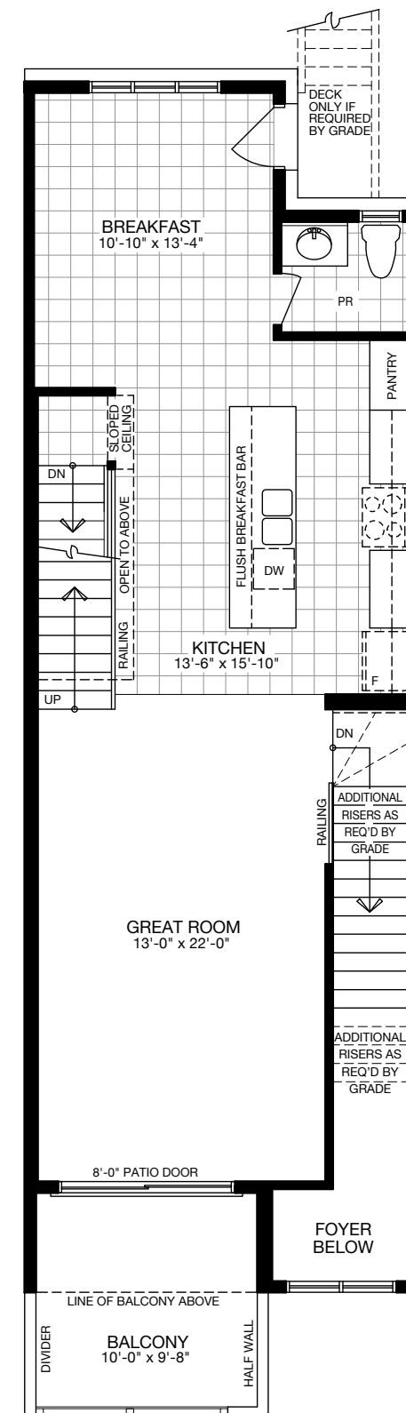
Main Floor Plan Elevation A & B
