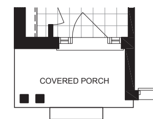
PARTIAL GROUND FLOOR PLAN ELEVATION B
